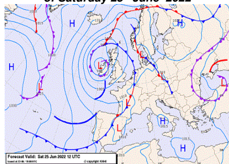
Sea surface prognostic chart for 12 GMT of Saturday 25 th June 2022
